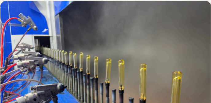
Automatic Coating Station
